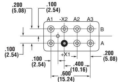
TERMINAL VIEW
