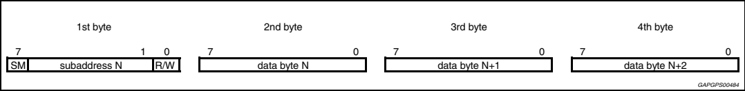
Figure 7. SPI
