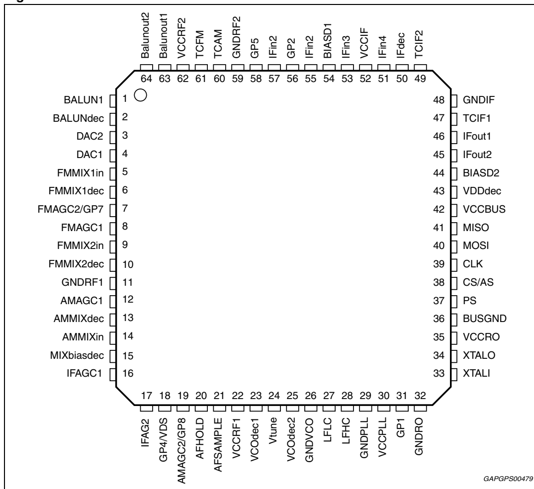
Figure 2. Pin connection
