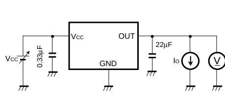
Fig.1 Measurement circuit for output voltage, input stability, load regulation, temperature coefficient of output voltage
