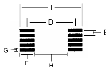
DEVICE FOOTPRINT
