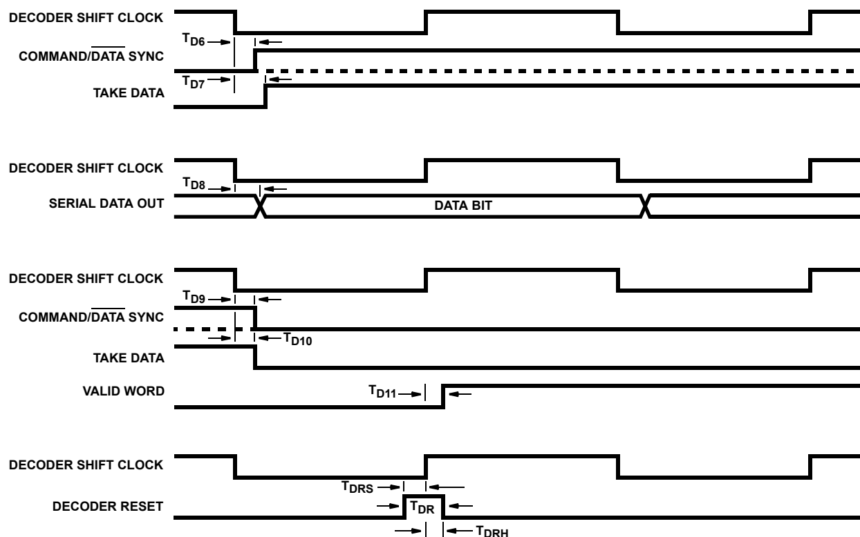
FIGURE 11. DECODER TIMING
