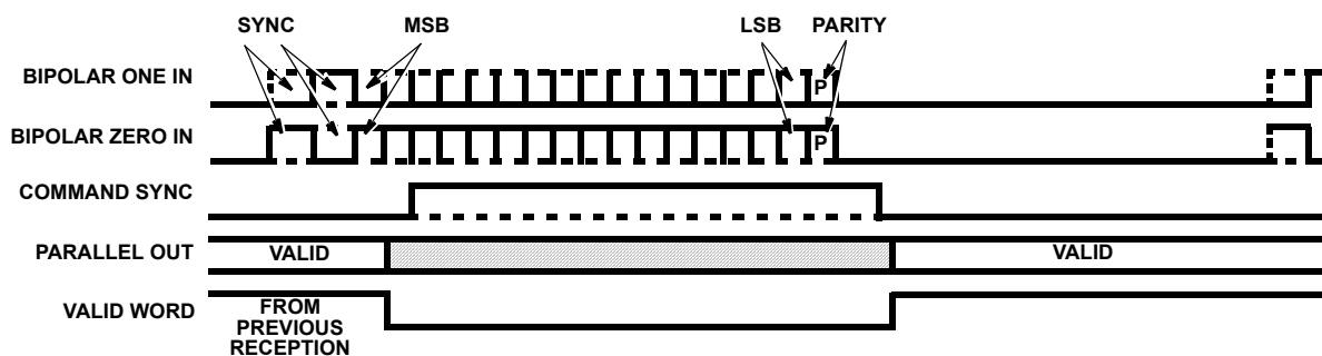
FIGURE 5. DECODER TIMING
