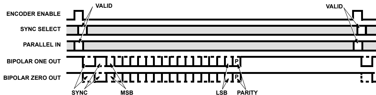
FIGURE 4. ENCODER TIMING
