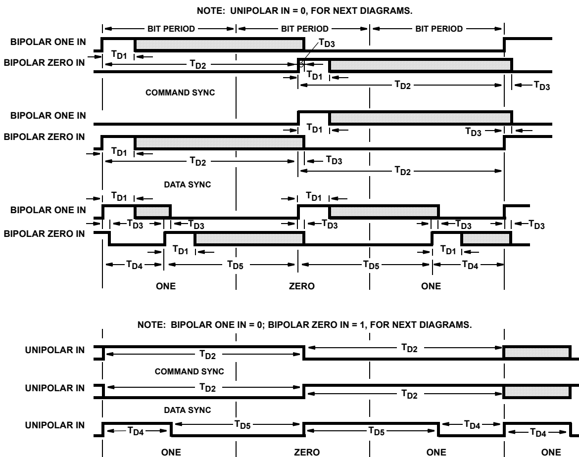
FIGURE 12. DECODER TIMING
