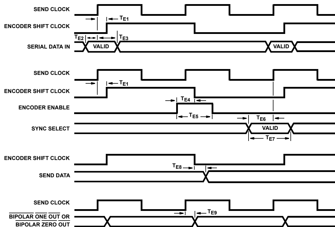
FIGURE 10. ENCODER TIMING
