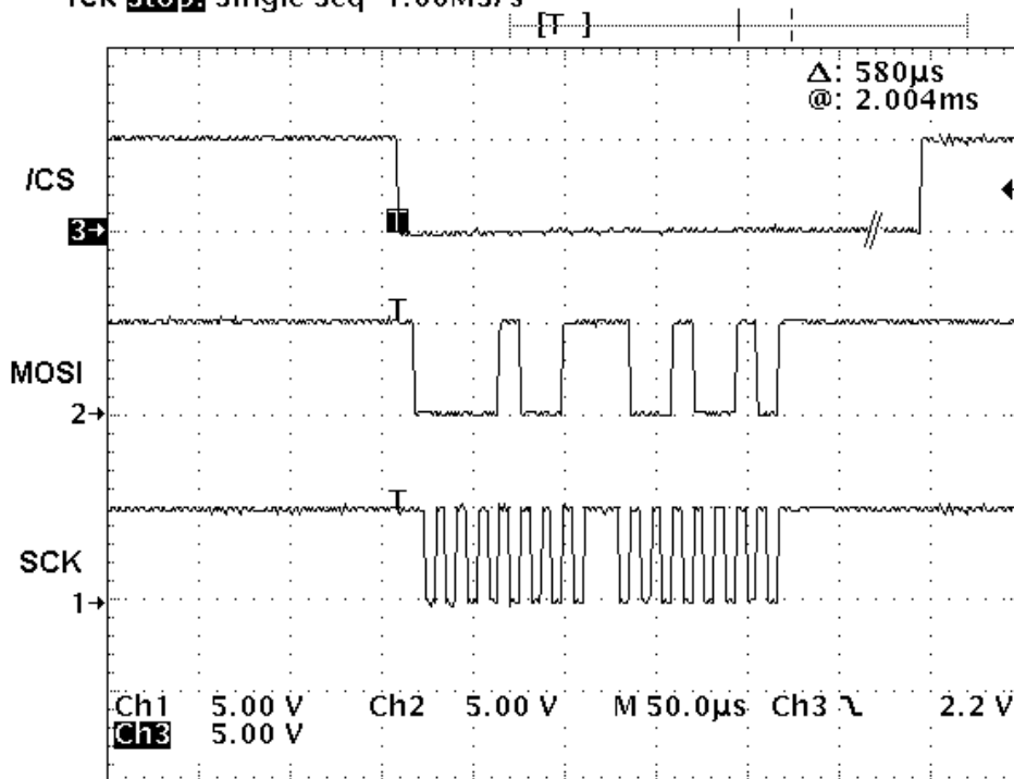
Figure 11: Scope Diagram. Value: 0000100110010010 bin / 0992 hex / 2450 dec ==&gt; 19.14 ln/min
