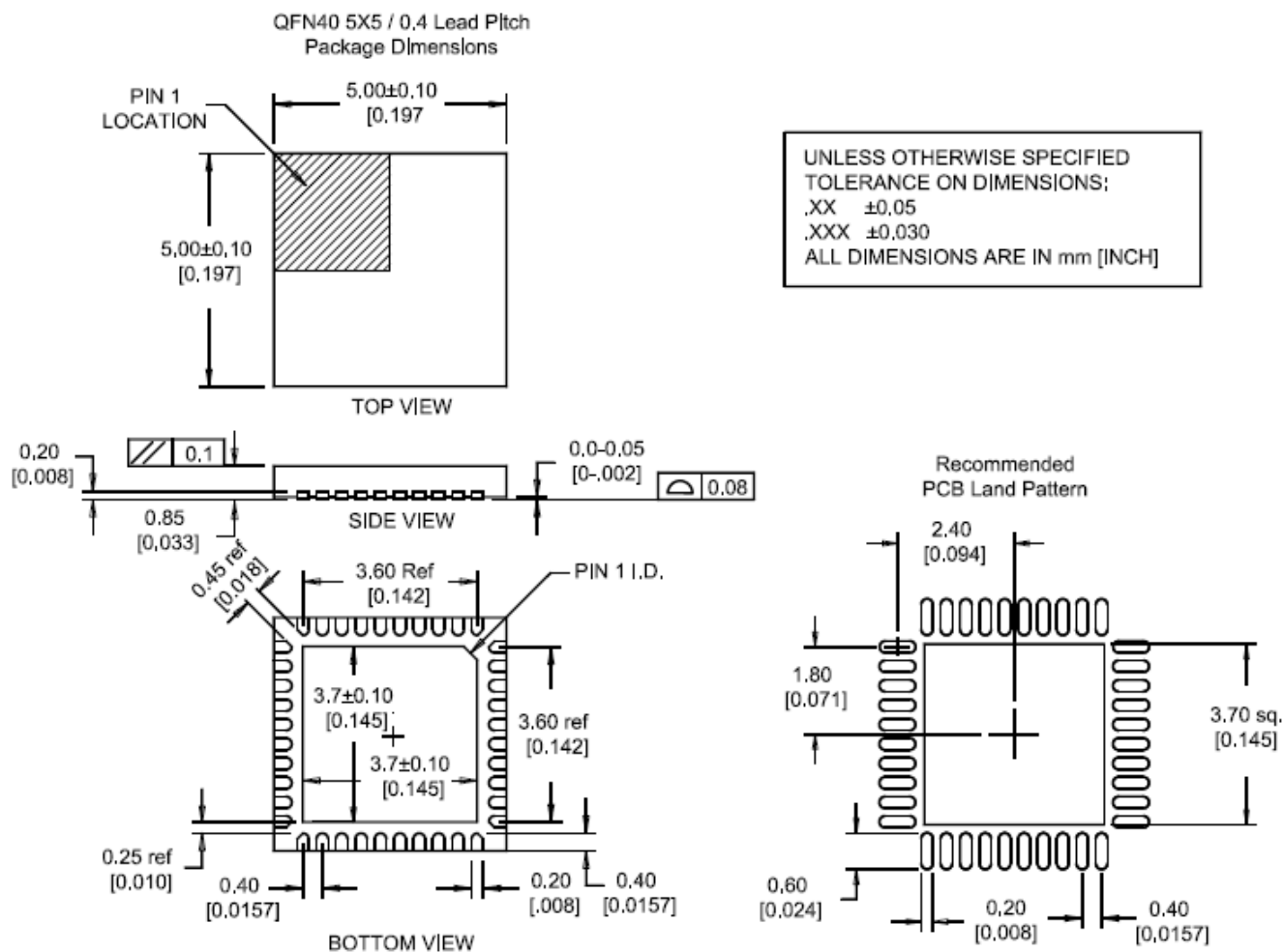
Figure 61: Package Dimensions
