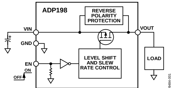
Figure 1. WLCSP
