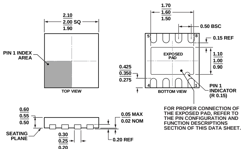
Figure 34. 8-Lead Lead Frame Chip Scale Package [LFCSP_UD] 2.00 × 2.00 mm Body, Ultra Thin, Dual Lead (CP-8-10)
