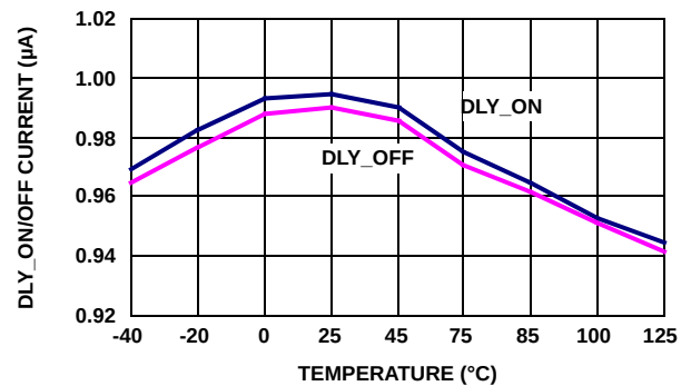
FIGURE 8. DLY CHARGE CURRENT
