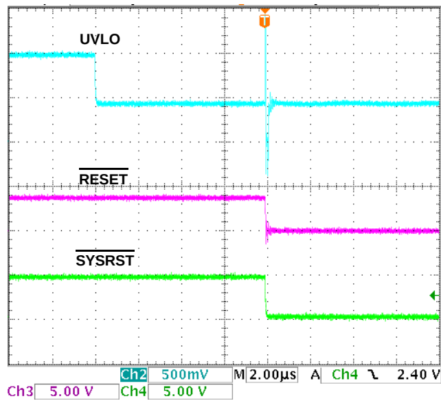
FIGURE 21. UVLO INVALID TO \overline{\text{RESET}} AND SYSRST LOW
