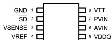
SO-8 Layout
