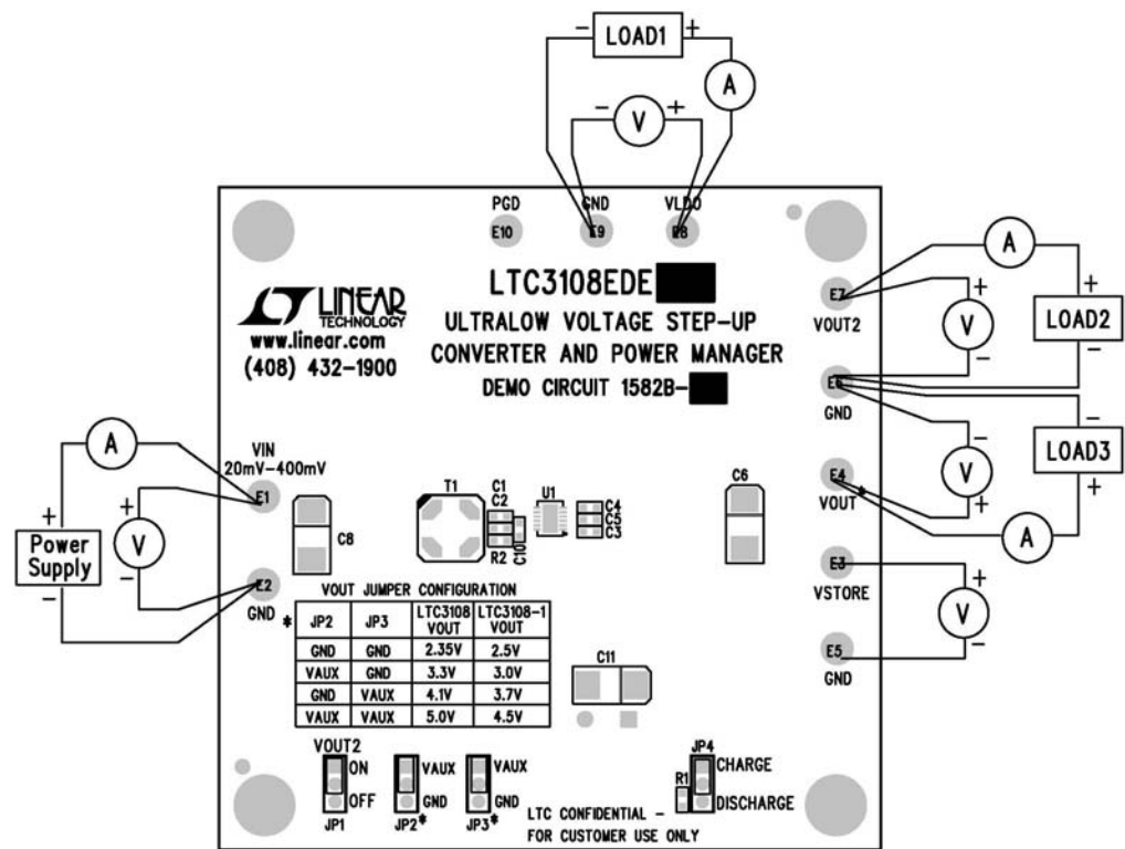
Figure 1. Connection Diagram
