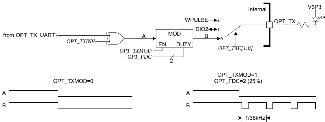
Figure 7: Optical Interface
