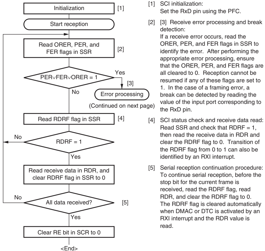
Figure 13.9 Sample Serial Reception Data Flowchart (1)
