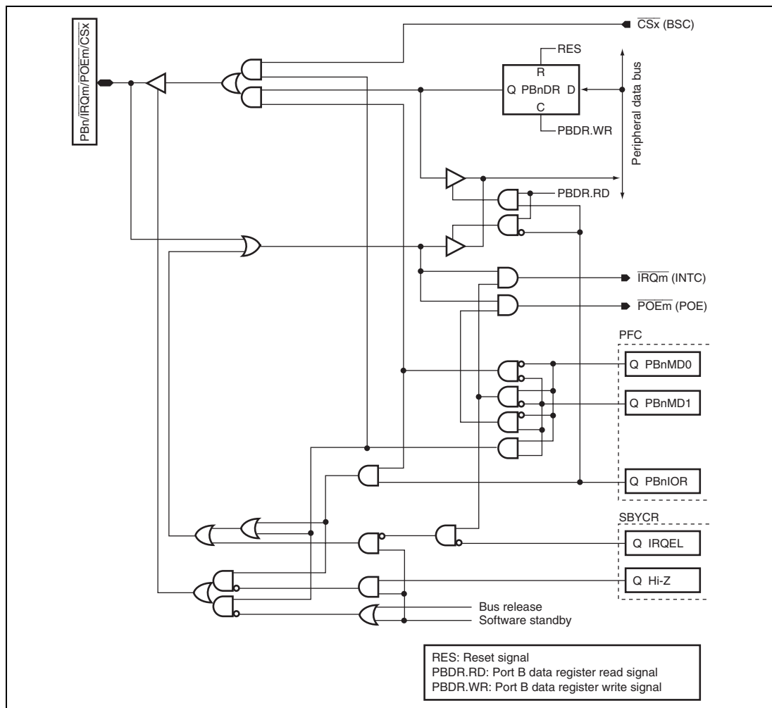
Figure D.17 \overline{\text{PBn/IRQm/POEm/CSx}}
