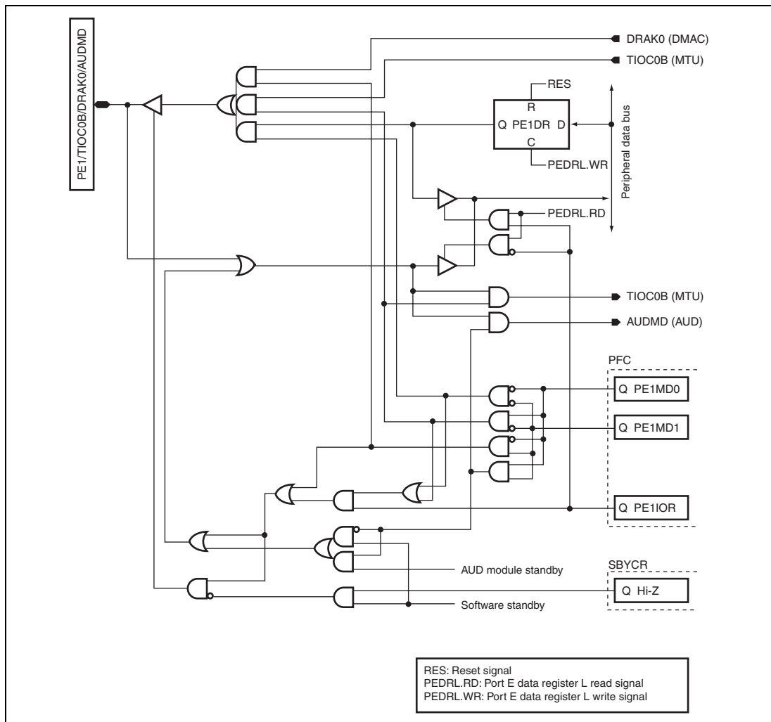
Figure D.47 PE1/TIOC0B/DRAK0/AUDMD
