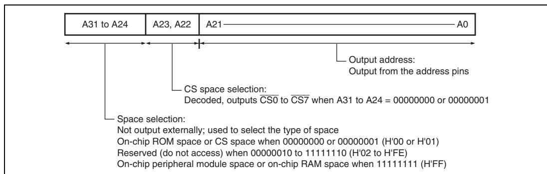
Figure 9.2 Address Format
