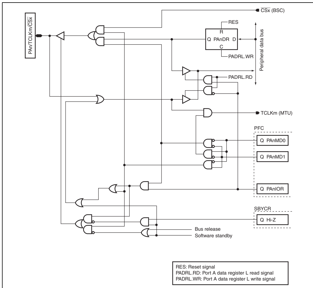
Figure D.4 PAn/TCLKm/ \overline{\text{CSx}}
