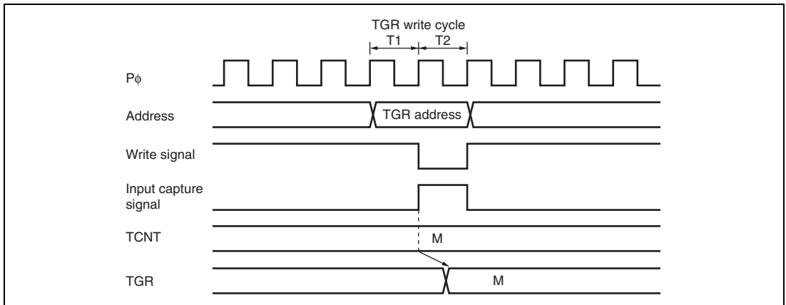
Figure 11.77 Contention between TGR Write and Input Capture
