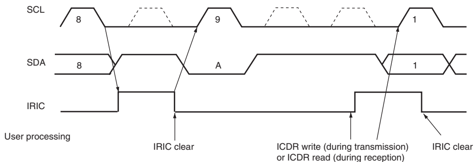
(b) When data transfer ends with ICDRE = 1 at transmission, or ICDRF = 1 at reception.
