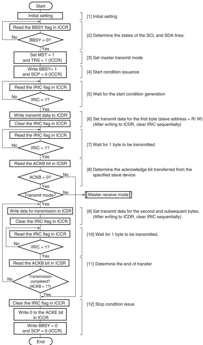
Figure 14.7 Example: Flowchart of Operations in the Master Transmit Mode
