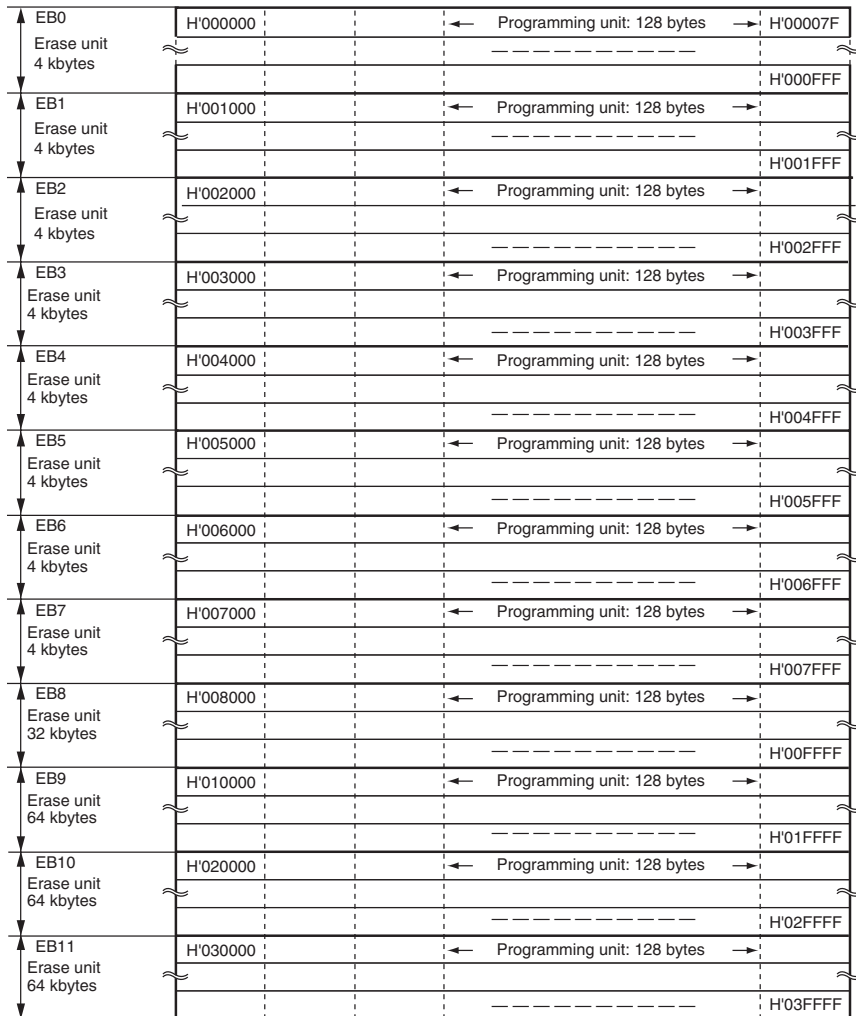
Figure 19.5 Flash Memory Block Configuration
