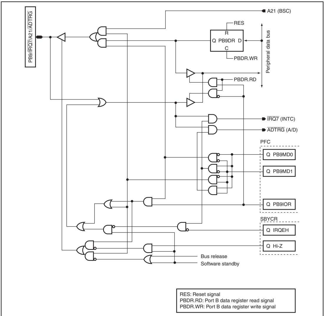
Figure D.21 PB9/ \overline{\text{IRQ7}} /A21/ \overline{\text{ADTRG}}
