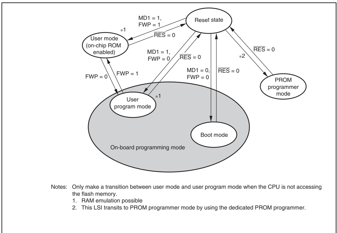
Figure 19.2 Flash Memory State Transitions
