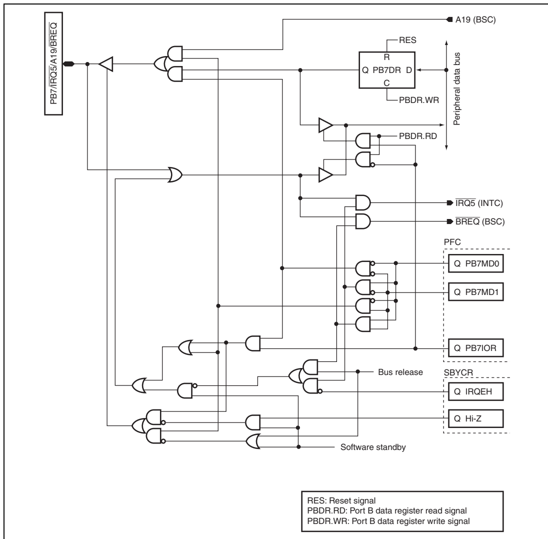
Figure D.19 PB7/ \overline{\text{TRQ5}} / \overline{\text{A19}} / \overline{\text{BREQ}}
