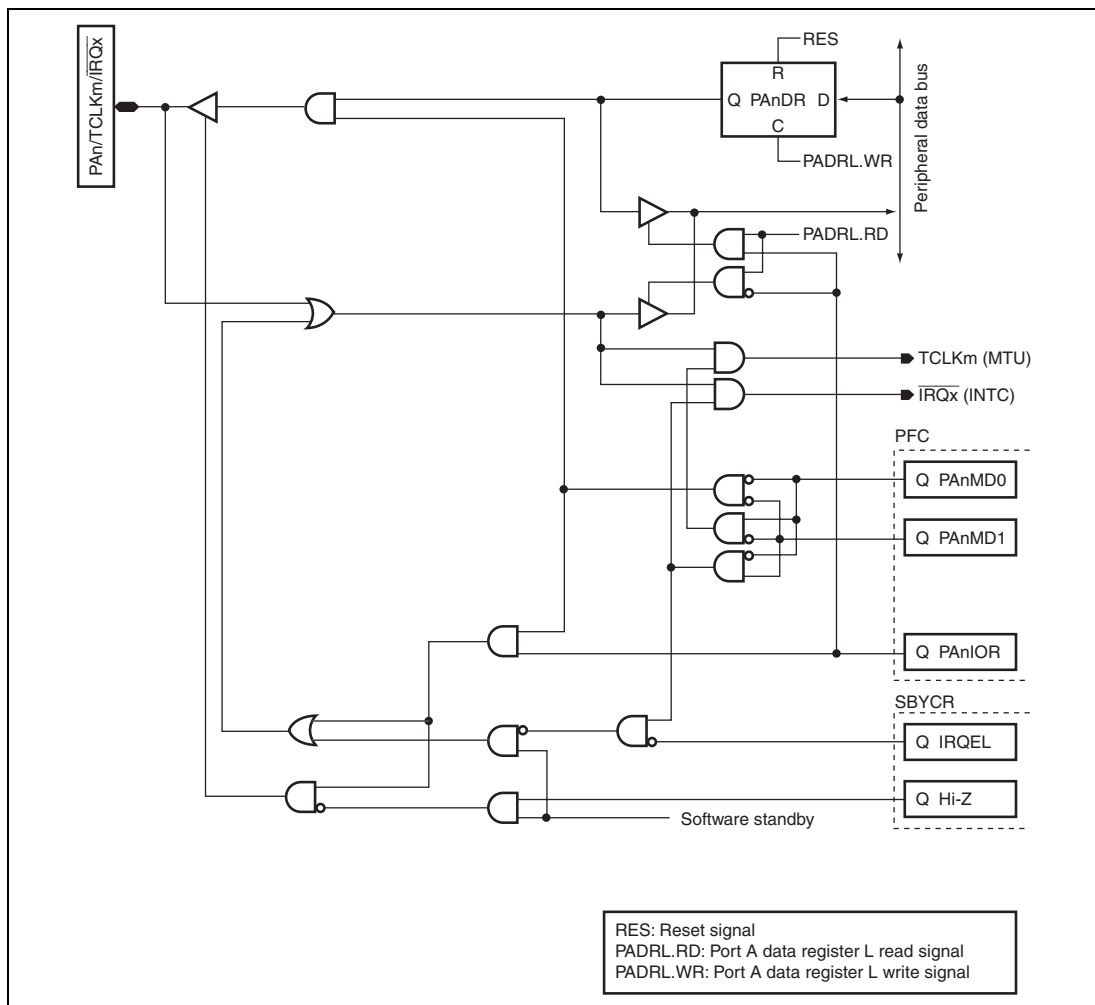
Figure D.5 PAn/TCLKm/IRQx
