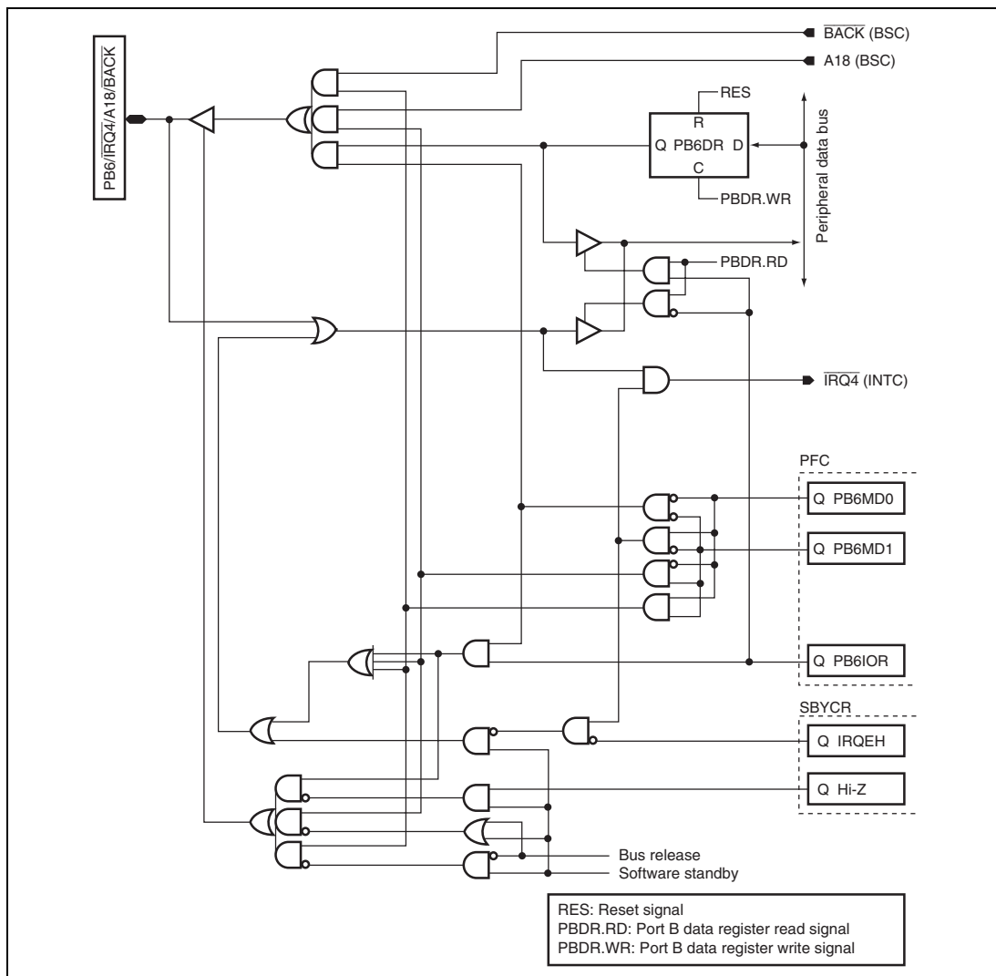
Figure D.18 PB6/IRQ4/A18/BACK
