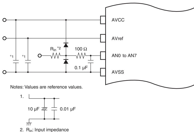
Figure 15.7 Example of Analog Input Protection Circuit
