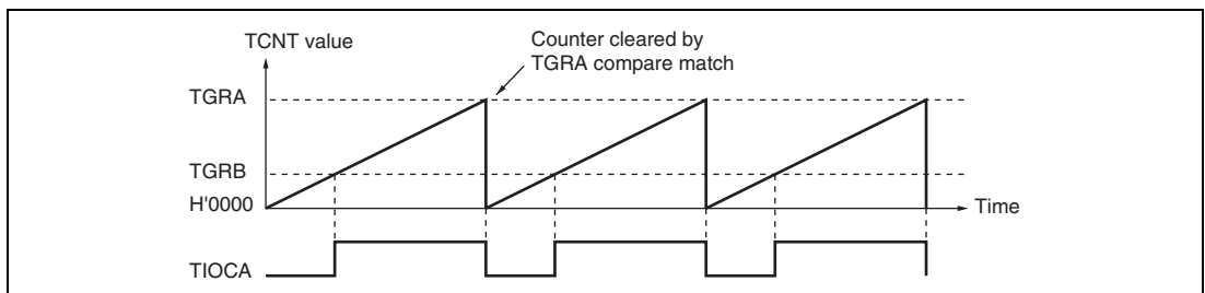
Figure 11.21 Example of PWM Mode Operation (1)
