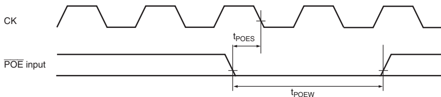
Figure 26.22 \overline{\text{POE}} Input/Output Timing
