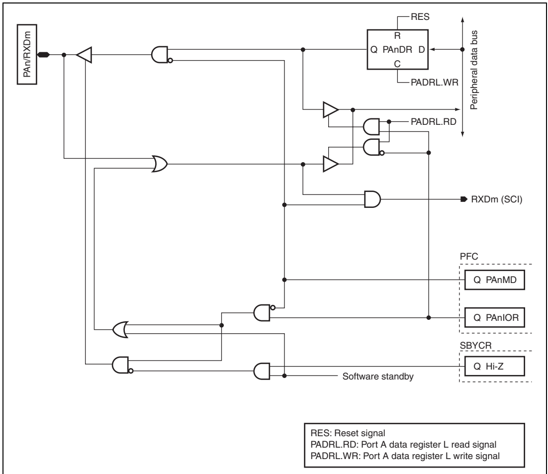
Figure D.1 PA0/RXD0
