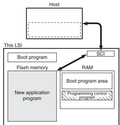
Figure 19.3 Boot Mode
