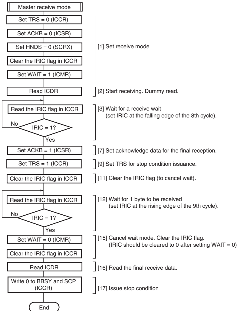
Figure 14.14 Example: Flowchart of Operations in Master Receive Mode (One Byte Reception) (WAIT = 1)
