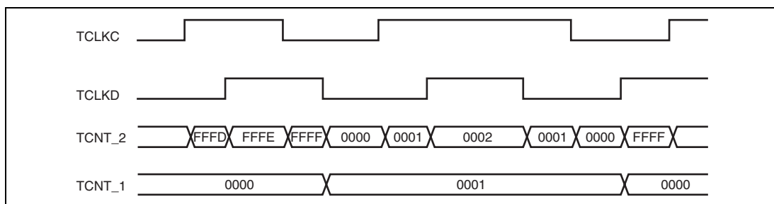
Figure 11.19 Example of Cascaded Operation
