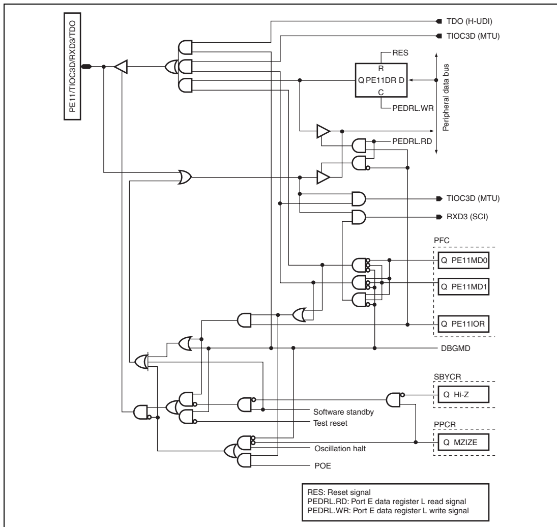
Figure D.55 PE11/TIOC3D/RXD3/TDO
