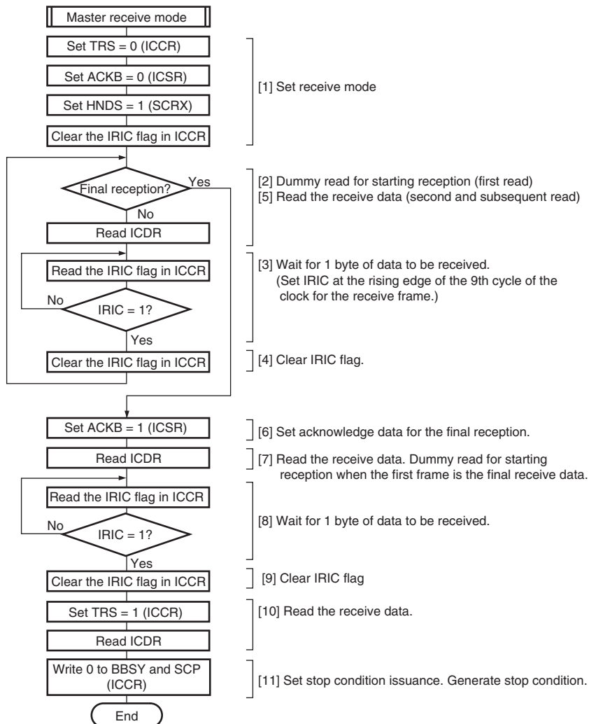
Figure 14.10 Example: Flowchart of Operations in the Master Receive Mode (HNDS = 1)
