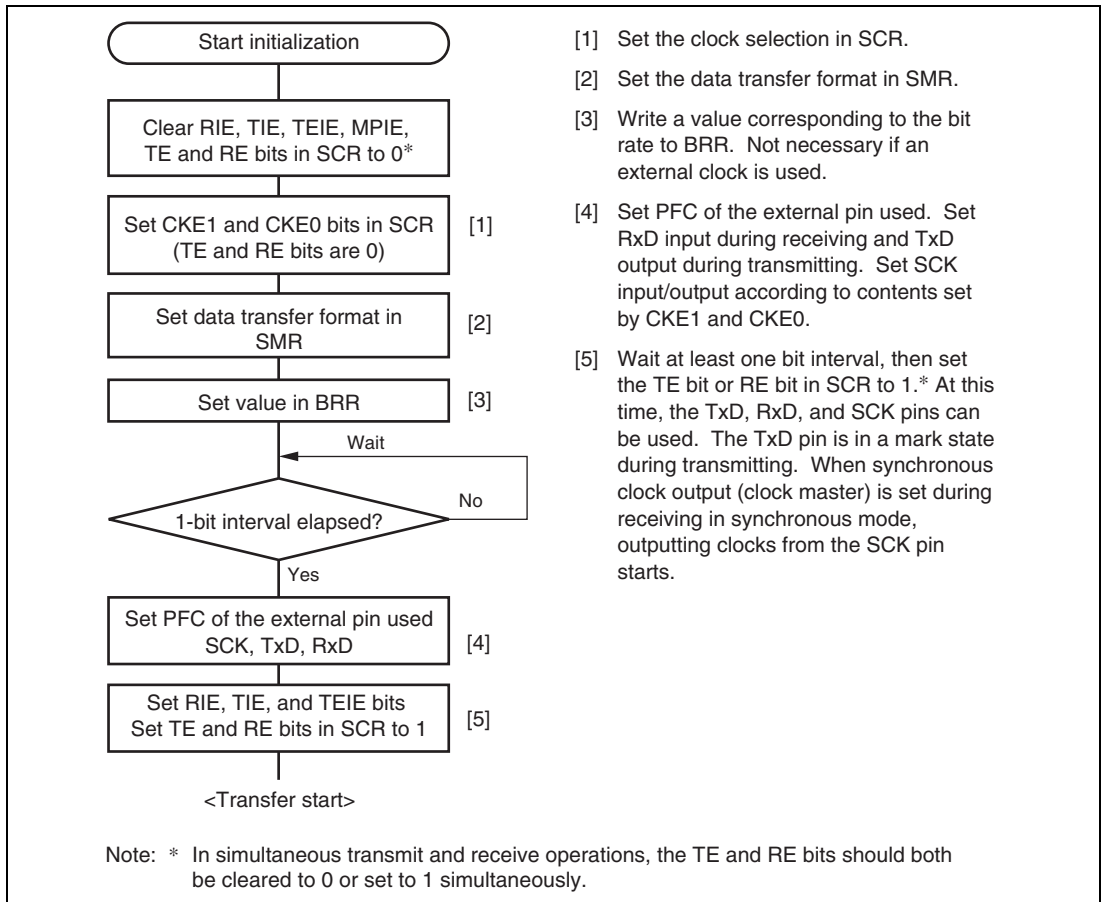
Figure 13.15 Sample SCI Initialization Flowchart
