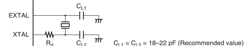
Figure 4.2 Connection of Crystal Resonator (Example)
