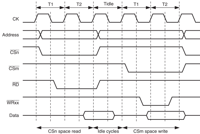
Figure 9.7 Example of Idle Cycle Insertion
