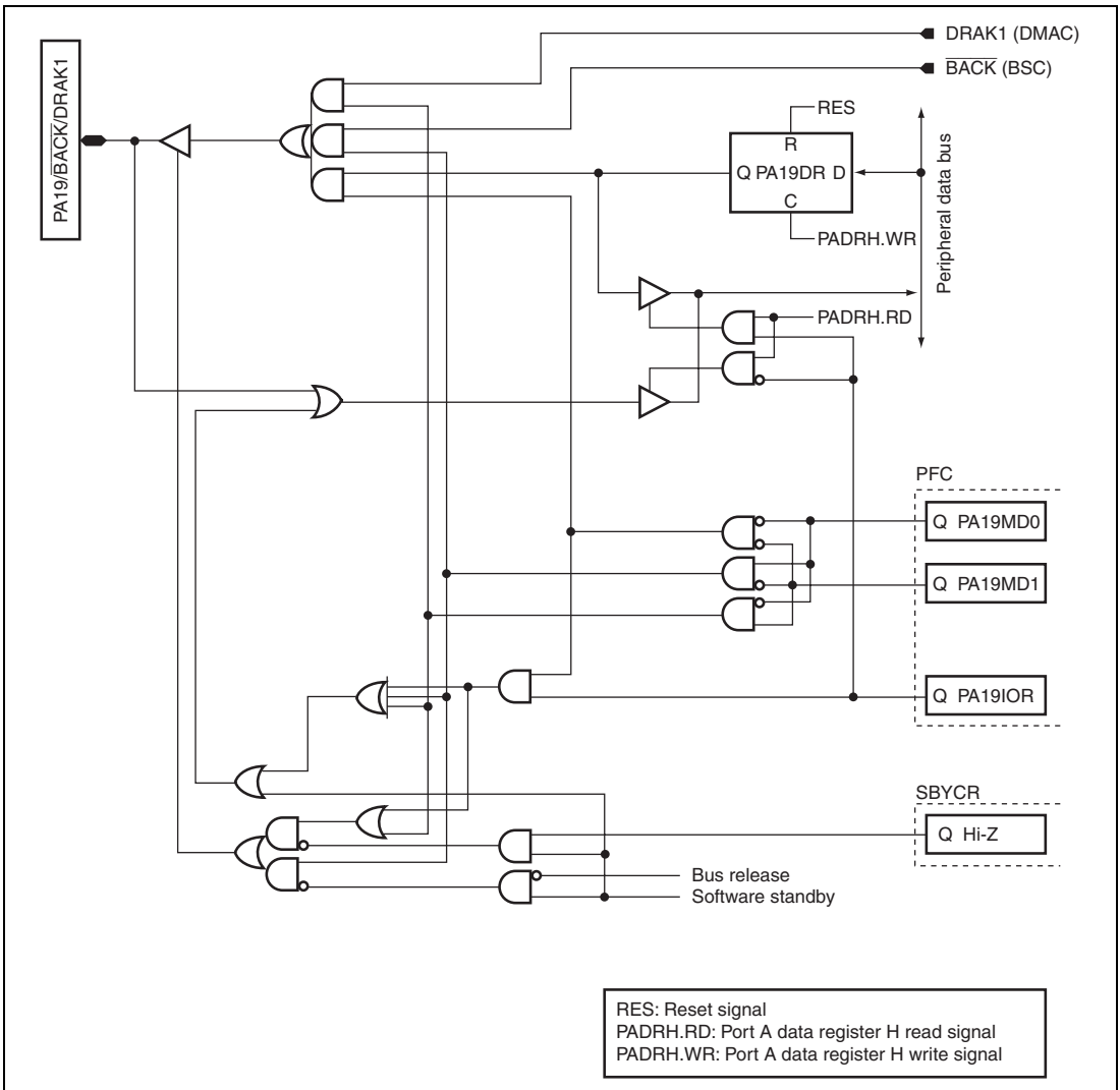
Figure D.11 PA19/ \overline{\text{BACK}} /DRAK1
