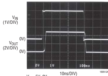
Output Overdriven Recovery
