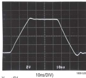
±5V Large-Signal Response
