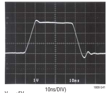
5V Large-Signal Response
