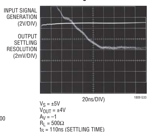
0.01% Settling Time
