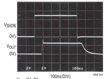
Shutdown Response
