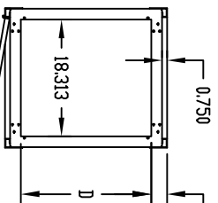
TOP VIEW (LESS TOP COVER & TOP COWLS)
