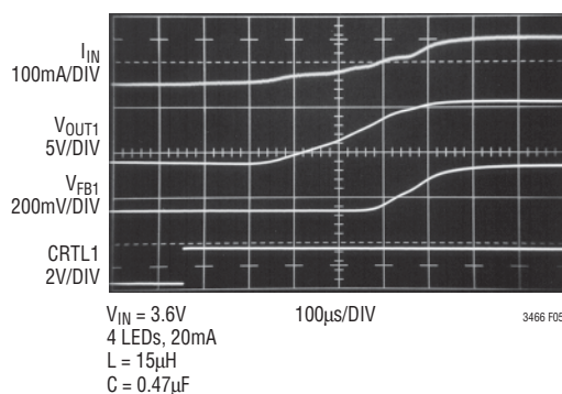
Figure 5. Start-Up Waveforms
