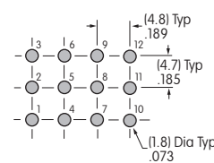
Four Pole
