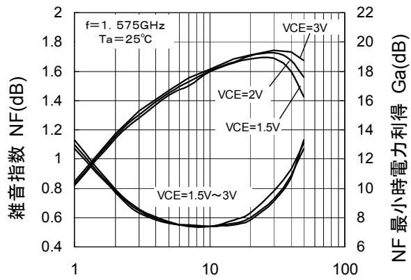
NF, Ga-IC
