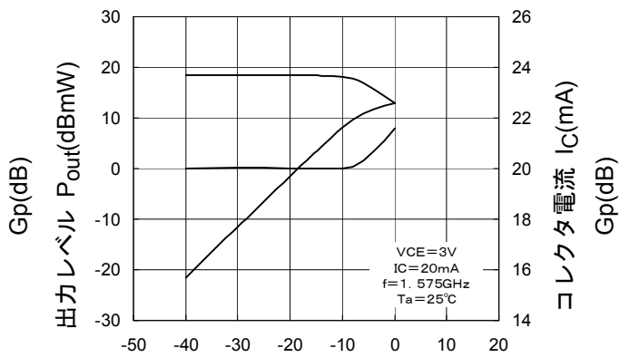
P_{out}, G_p, I_C - P_{in}
