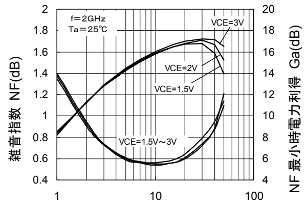
NF, Ga-IC
