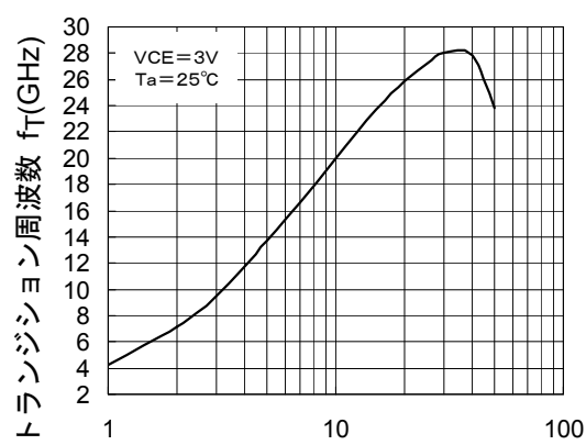
f_T-I_C
