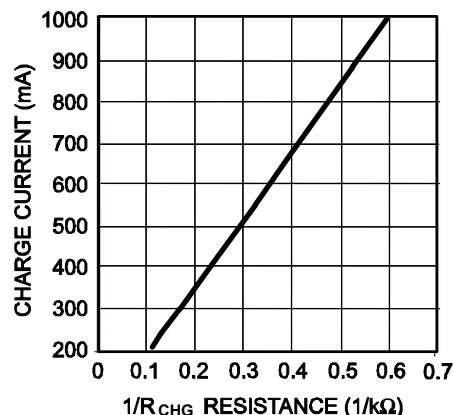
Figure 4—Charge Current vs 1/R_{CHG} Resistance
