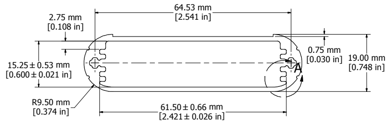
EXTRUSION
