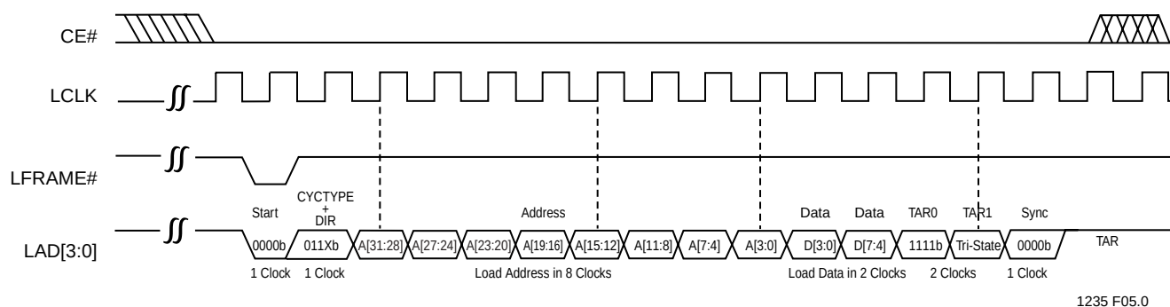
FIGURE 5: LPC WRITE CYCLE WAVEFORM
