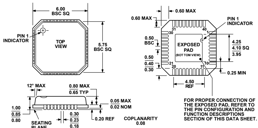
Figure 48. 40-Lead Lead Frame Chip Scale Package [LFCSP_VQ] 6 mm × 6 mm Body, Very Thin Quad (CP-40-1)
