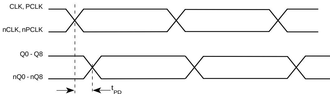
FIGURE 7 - PROPAGATION DELAY
