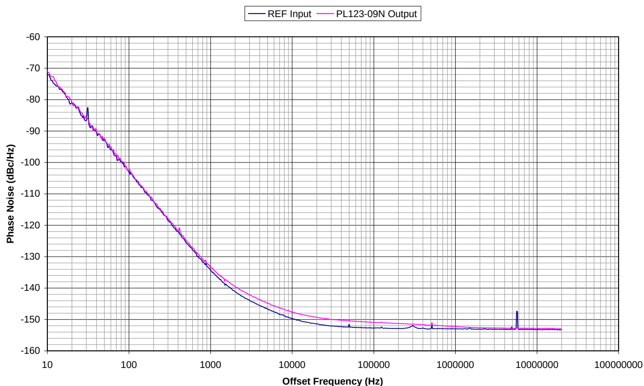
PL123-09N Additive Phase Jitter: V DD =3.3V, CLK=100MHz, Integration Range 12KHz to 20MHz: 0.059ps typical.
