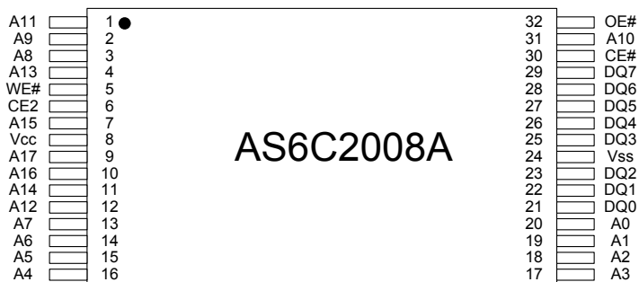
TSOP-I/STSOP
