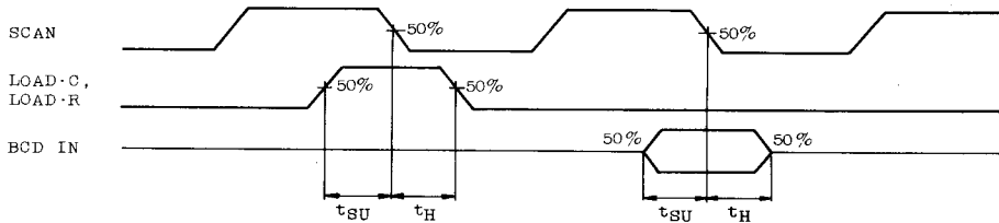
WAVEFORM 4
