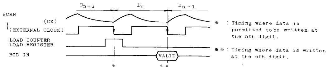
LOAD REGISTER, LOAD COUNTER TIMING CHART
