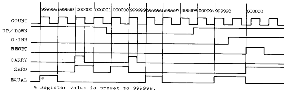
DIGIT COUNTER TIMING CHART
