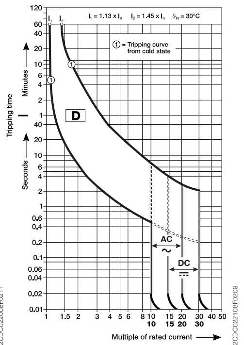
D characteristic
