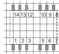
RECOMMENDED FOOTPRINT Bottom view, grid: 2.54mm (0.1inch)
