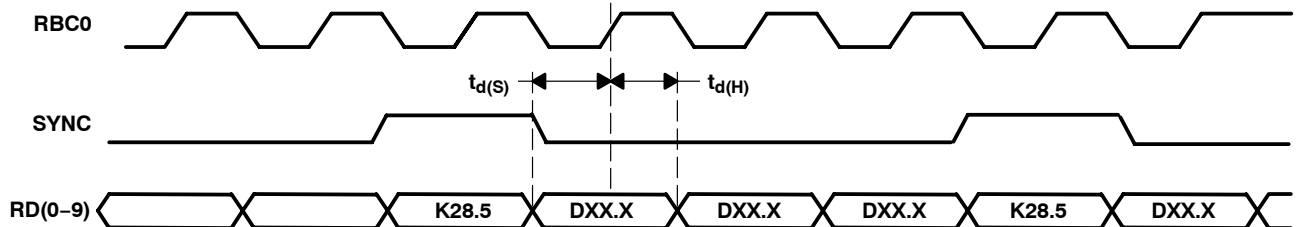
Figure 3. Synchronous Timing Characteristics Waveforms (TBI full-rate mode)
