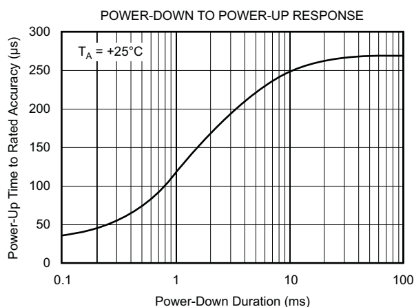
Figure 46. Power-Down to Power-Up Response
