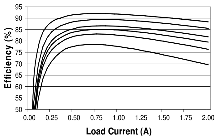
Efficiency vs. Load Current ( V_{in} = 5.0\text{V} )
