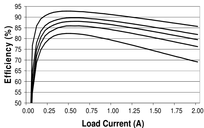
Efficiency vs. Load Current ( V_{in} = 3.3\text{V} )
