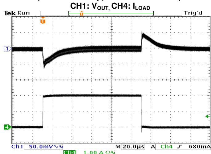
Transient Response at V_{IN} = 5\text{ V} V_{OUT} = 3.3\text{ V} , C_{OUT} = 1 \times 47\text{ }\mu\text{F} (0-2 A Load Step, slew rate \geq 10\text{ A}/\mu\text{s} ) CH1: V_{OUT} , CH4: I_{LOAD}
