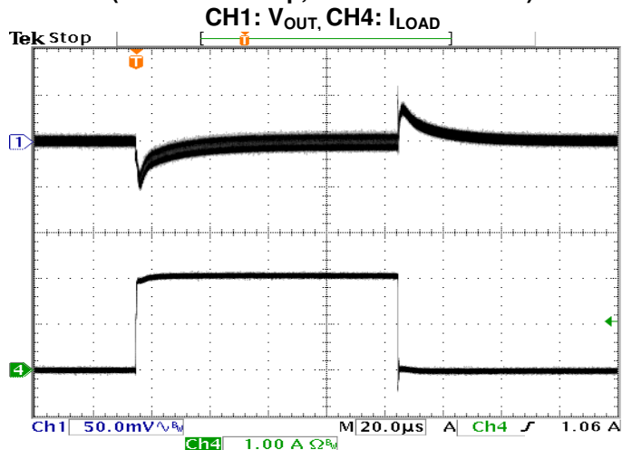
Transient Response at V_{IN} = 5\text{ V} V_{OUT} = 1.2\text{ V} , C_{OUT} = 1 \times 47\text{ }\mu\text{F} (0-2 A Load Step, slew rate \geq 10\text{ A}/\mu\text{s} ) CH1: V_{OUT} , CH4: I_{LOAD}
