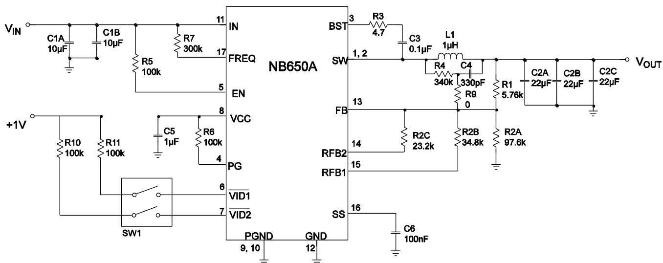
Figure 15: Typical Application Circuit V_{IN} = 19V , V_{OUT} = 0.65/0.75/0.80/0.90V , I_{OUT} = 6A
