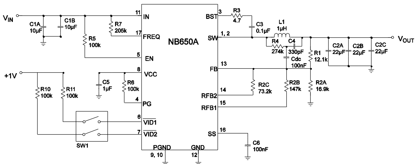
Figure 14: Typical Application Circuit with Low-ESR Ceramic Capacitor and DC-Blocking Capacitor V_{IN} = 12V , V_{OUT} = 1.05/1.10/1.15/1.20V , I_{OUT} = 6A , f_{SW} = 550kHz
