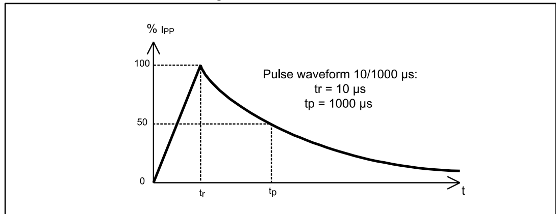
Figure 3: Pulse waveform
