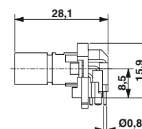
M12 pin contact carrier, angled, 8-pos.
