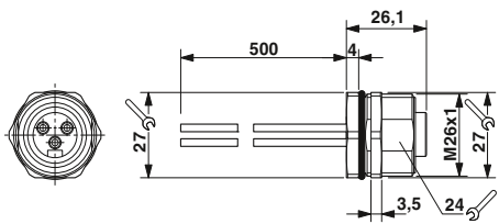
7/8" flush-type socket
