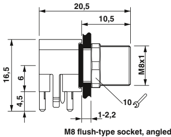
M8 flush-type socket, angled
