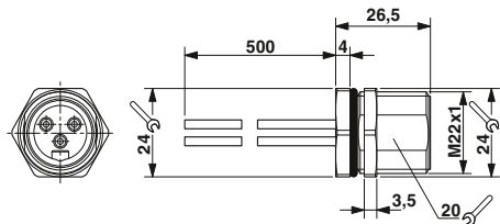
7/8" flush-type plug
