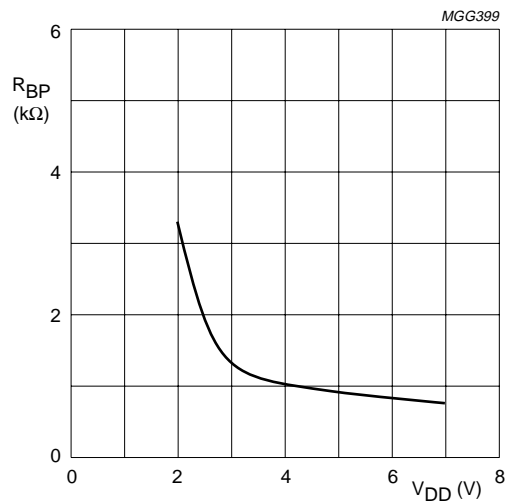
a. Backplane output impedance BP0 to BP3 ( R_{BP} ); V_{DD} = 5 V; T_{amb} = -40 to +85^{\circ}C .
