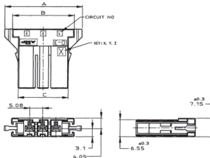
Panel/Free-hanging Type
