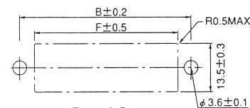
Panel Cutout
