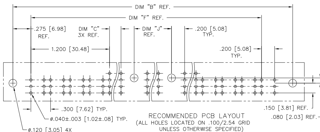
DETAIL P (INSTALLED IN PCB, NOTE 8)
