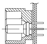
DETAIL P (INSTALLED IN PCB, NOTE 8)
