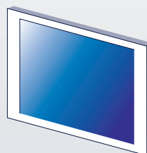
PLASMA
