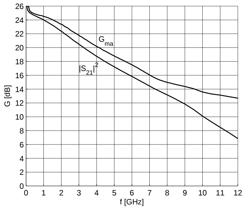
Figure 7-4 Gain G_{ma} , G_{ms} , |S_{21}|^2 = f(f) , V_{CE} = 1.8 V, I_C = 15 mA
