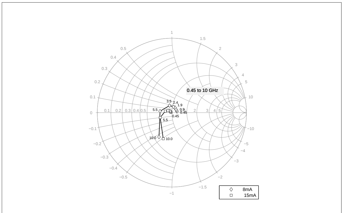
Figure 7-8 Source Impedance for Minimum Noise Figure Z_{opt} = f(f) , V_{CE} = 1.8 V, I_C = 8 / 15 mA
