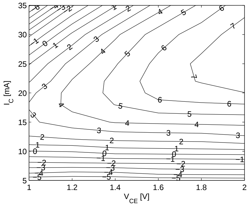
Figure 7-3 Compression Point at Output OP_{1dB} [dBm] = f(I_C, V_{CE}) , Z_S = Z_L = 50 \Omega , f = 5.5 GHz
