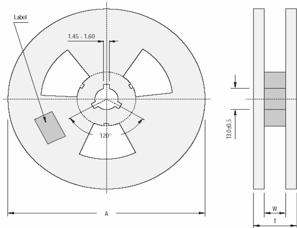
Reel Specifications
