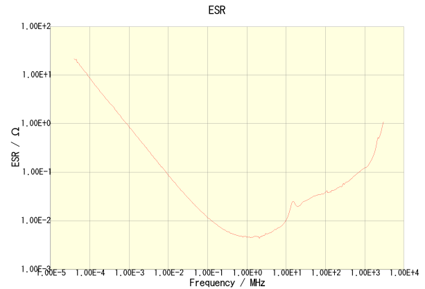
C3216X7R2A105K160AA
