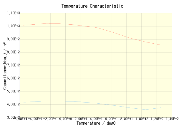
C3216X7R2A105K160AA(DC Bias = 0V) C3216X7R2A105K160AA(DC Bias = 50V)
