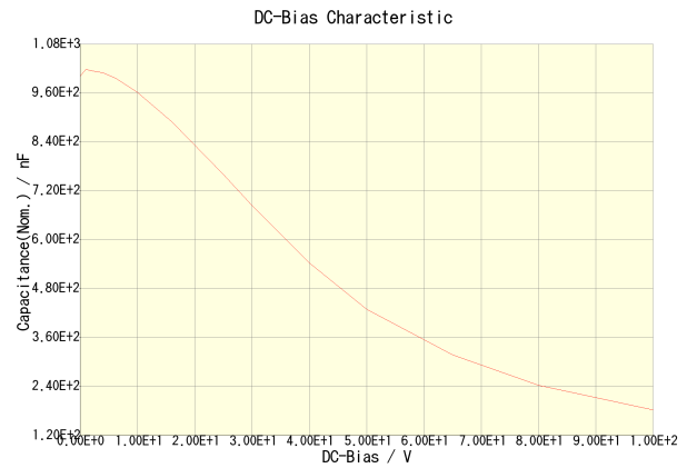
C3216X7R2A105K160AA
