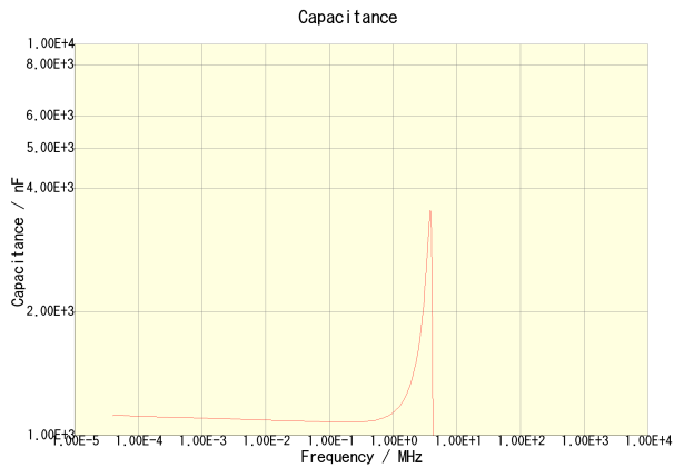
C3216X7R2A105K160AA
