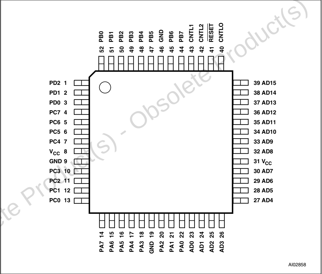
Figure 1. PQFP52 connections
