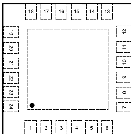
24-Lead WQFN Package (top view)
