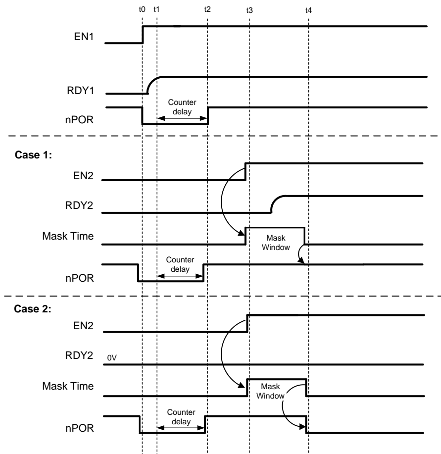
Figure 39. NPOR Mask Window
