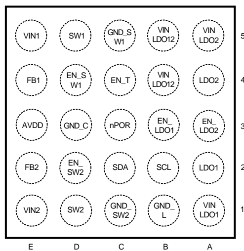
25-Bump Thin DSBGA Package, Large Bump Package Number YZR0025, Bottom View
