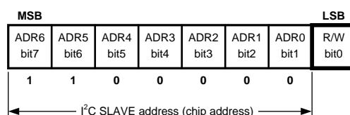
Figure 43. I 2 C Chip Address (see note above)
