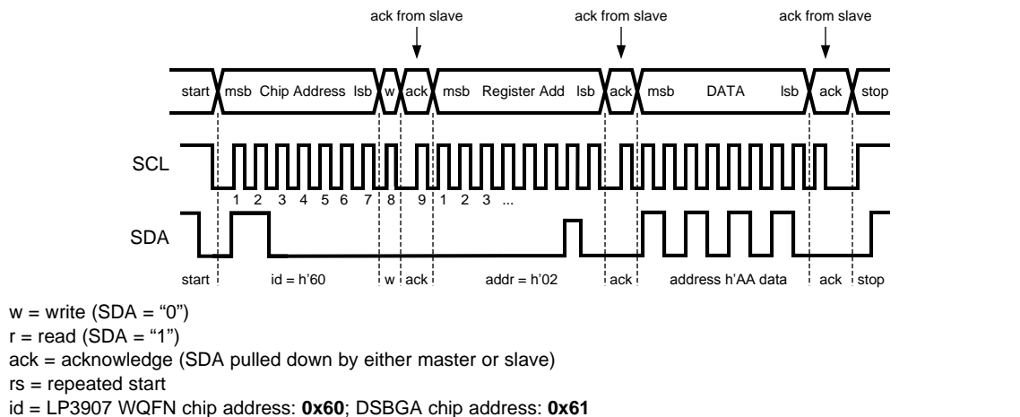
Figure 44. I²C Write Cycle
