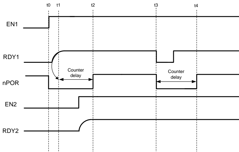
Figure 38. Faults Occurring in Counter Delay After Startup
