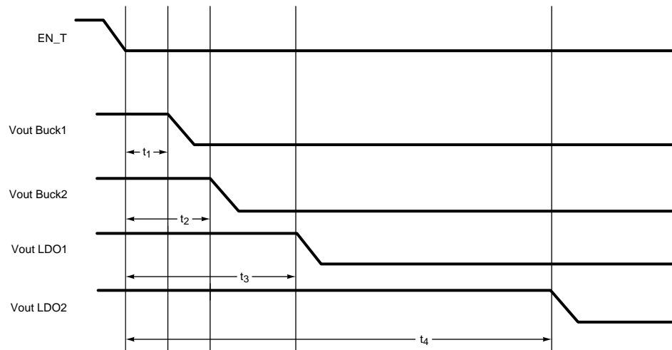
Figure 36. LP3907 Default Power-Off Sequence
