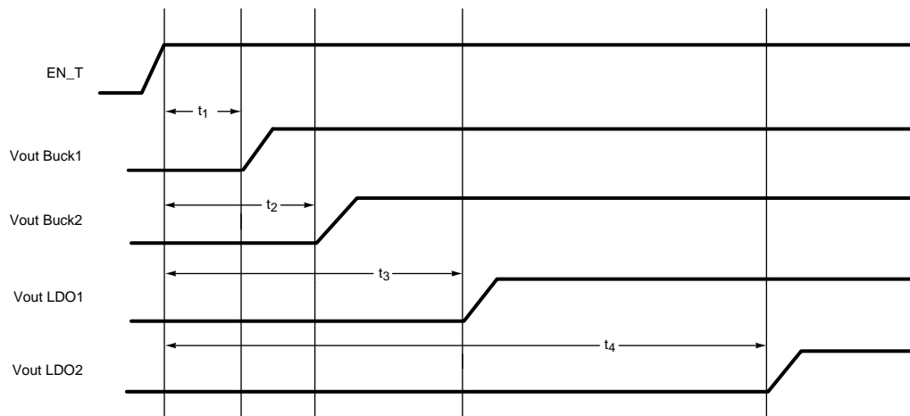
Figure 35. LP3907 Default Power-Up Sequence
