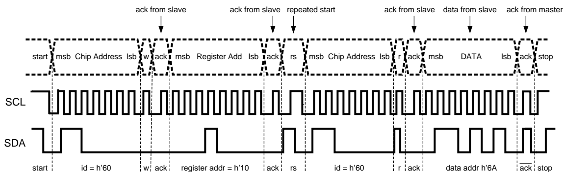
Figure 45. I²C Read Cycle
