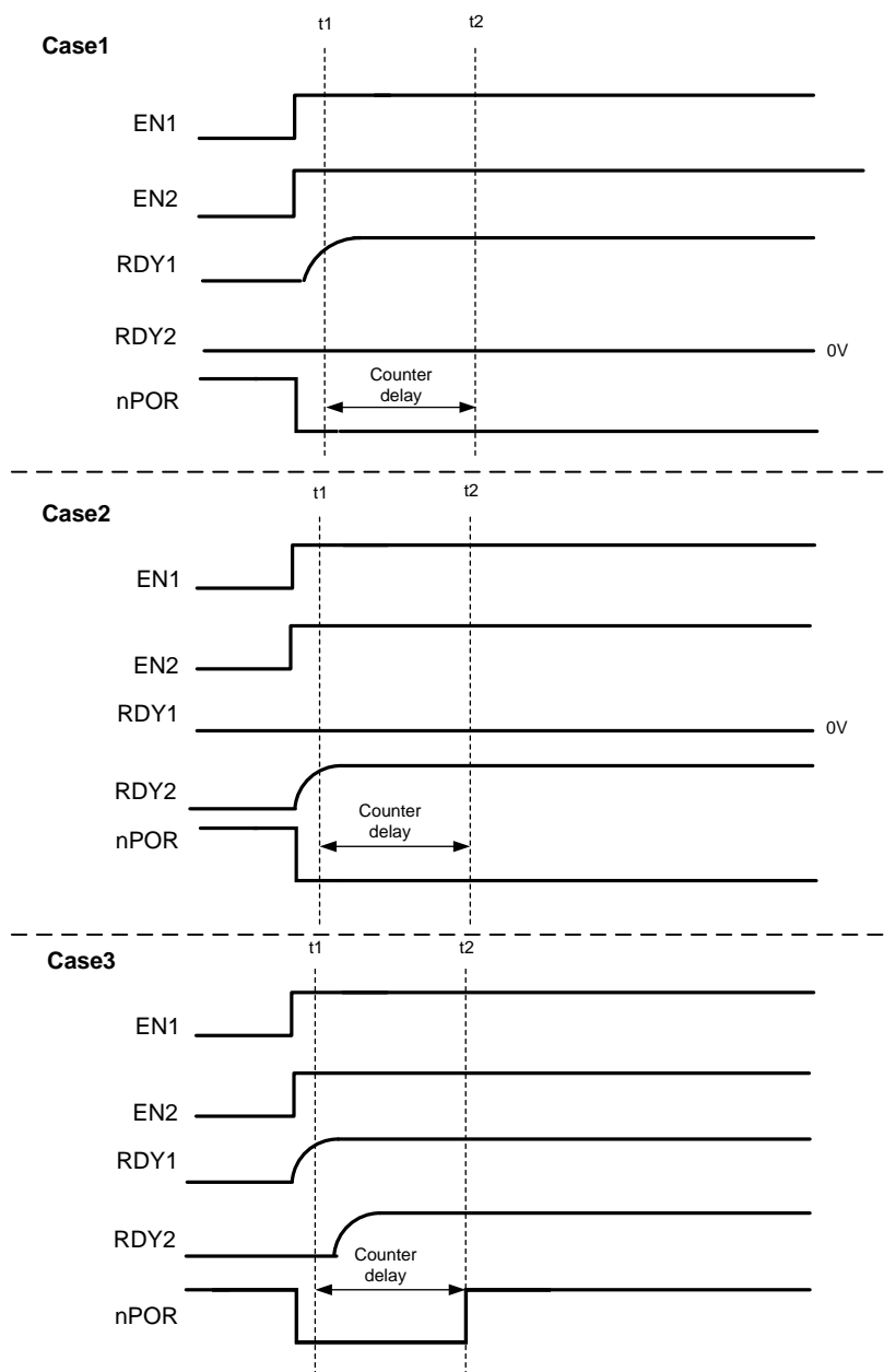
Figure 37. NPOR With Counter Delay
