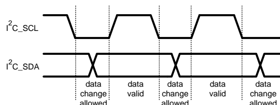
Figure 41. I 2 C Signals: Data Validity
