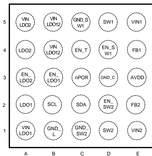
25-Bump Thin DSBGA Package, Large Bump Package Number YZR0025, Top View
