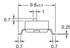
Raised Actuator
