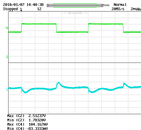
Figure 44 – Transient Response, 230 VAC, 75% \leftrightarrow 100% Step Load. Top: Load Current, 0.5 A / div. Bottom: V_{OUT} , 100 mV / div. Time Scale: 2 ms / div.
