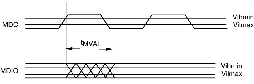
Figure 62. Management Data Output Valid Delay Timing
