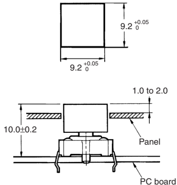
Panel Cutout
