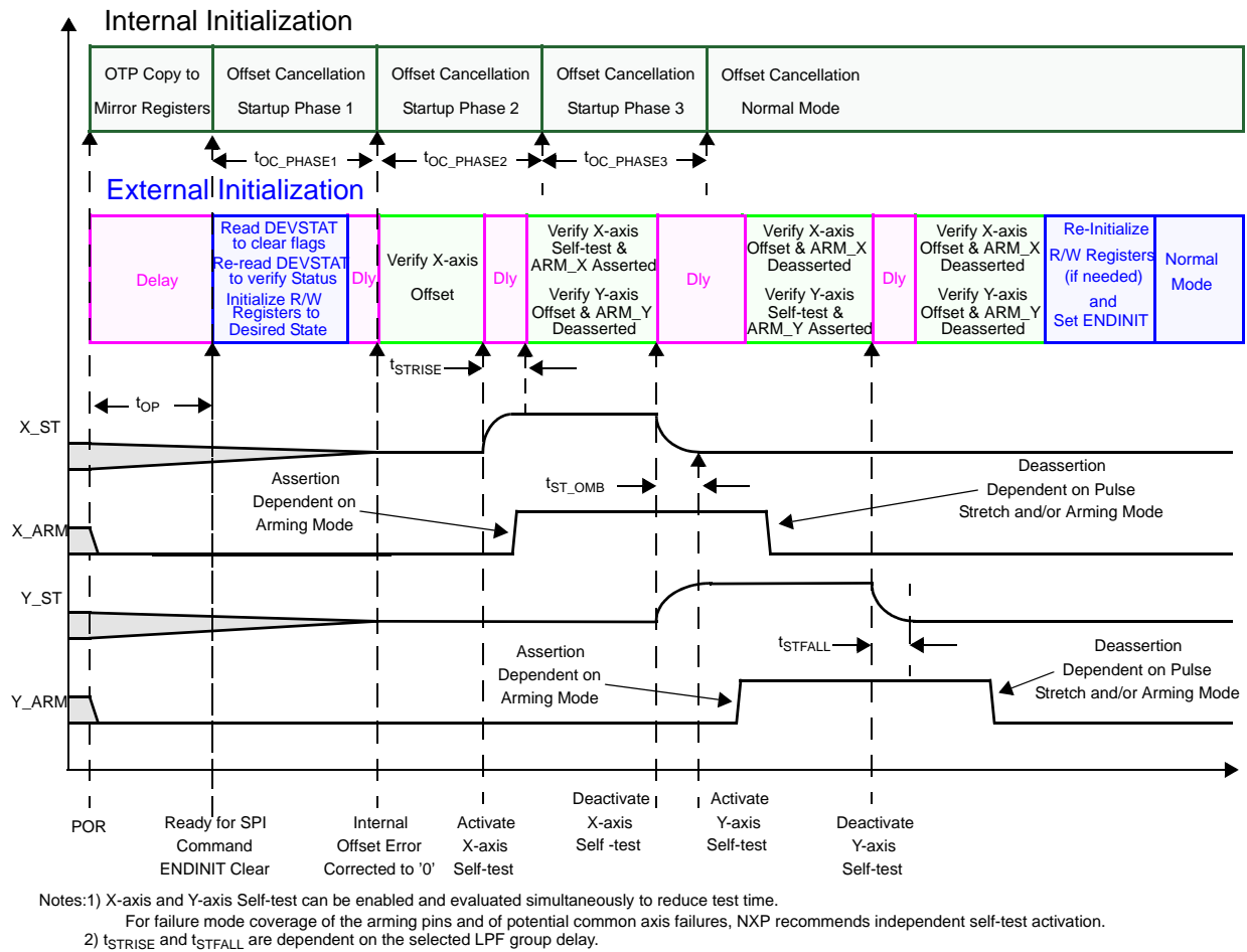
Figure 32. Initialization Process
