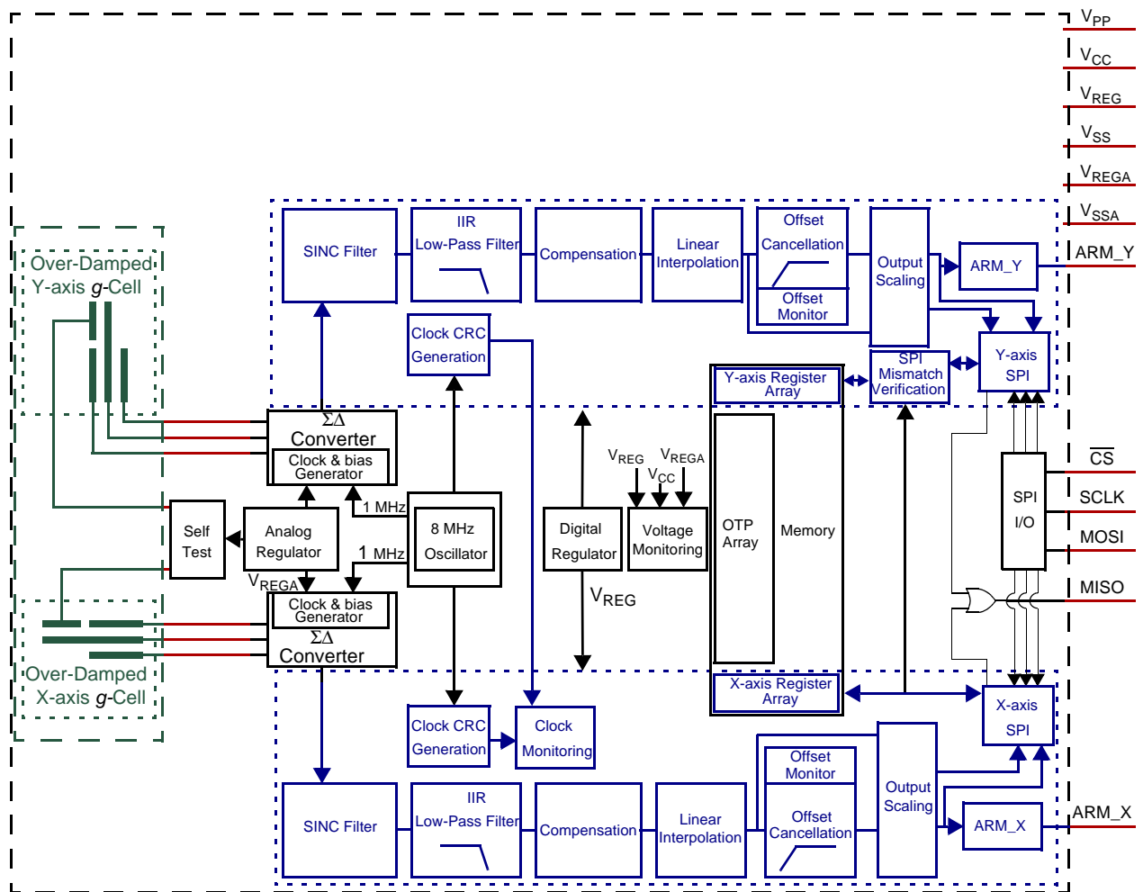
Figure 4. Block Diagram
