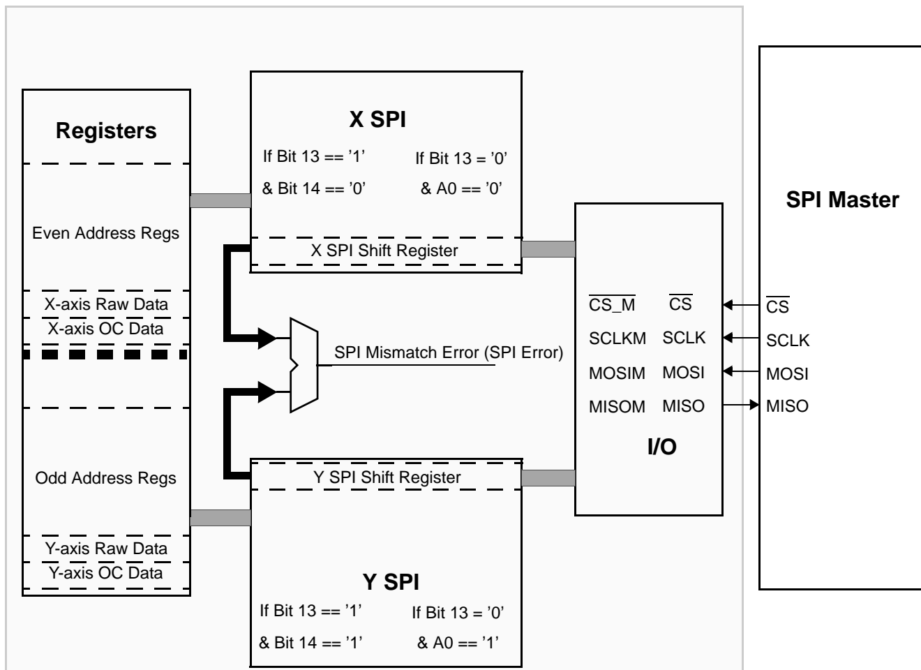
Figure 31. SPI Diagram
