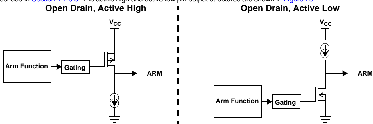
Figure 29. Arming Function - Pin Output Structure
