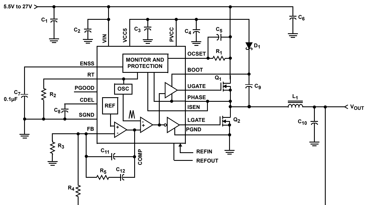
FIGURE 4. TYPICAL STEP DOWN DC/DC APPLICATION SCHEMATIC
