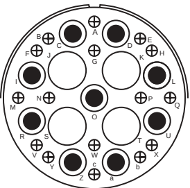
Insert Arrangement 40-10 Service Rating A Number of Contacts 4 9 16 Contact Size 4 8 16
