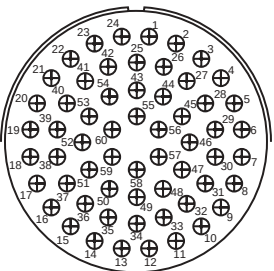
Insert Arrangement 40-53 Service Rating A Number of Contacts 60 Contact Size 16
