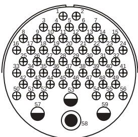
Insert Arrangement 40-61 Service Rating A Number of Contacts 1 3 55 Contact Size 8 12 16
