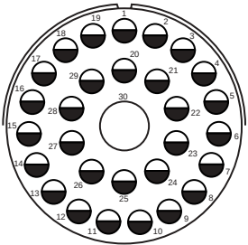
Insert Arrangement 40-30 Service Rating A Number of Contacts 29 1 Contact Size 12 4
