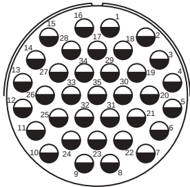
Insert Arrangement 40-35 Service Rating D Number of Contacts 35 Contact Size 12
