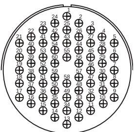
Insert Arrangement 40-62 Service Rating A Number of Contacts 60 Contact Size 16
