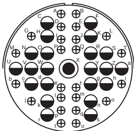
Insert Arrangement 40-9 Service Rating A Number of Contacts 1 22 24 Contact Size 8 12 16
