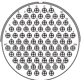
Insert Arrangement 40-56 Service Rating A Number of Contacts 85 Contact Size 16
