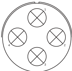
Insert Arrangement 40-57 Service Rating E Number of Contacts 4 Contact Size 0
